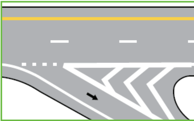
Figure 5.2 (FHWA/MUTCD: Figure 3B-8, pg. 548)
